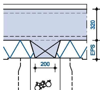
DETAIL 4 - RAVEELOPLEGGING
