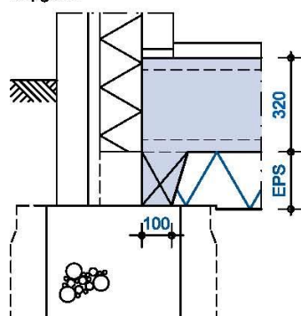
DETAIL 2 - RANDOPLEGGING
