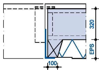
DETAIL 4 - RAVEELOPLEGGING
