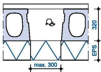
DETAIL 5 - EPS PASSTROOK
