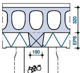
DETAIL 5 - EPS PASSTROOK
