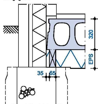
DETAIL 3 - TUSSENOPLEGGING
