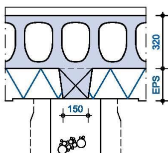
DETAIL 5 - EPS PASTROOK
