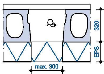
DETAIL 5 - EPS PASTROOK
