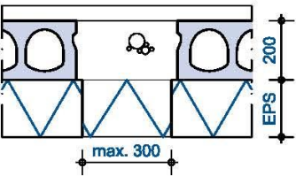
DETAIL 5 - EPS PASSTROOK
